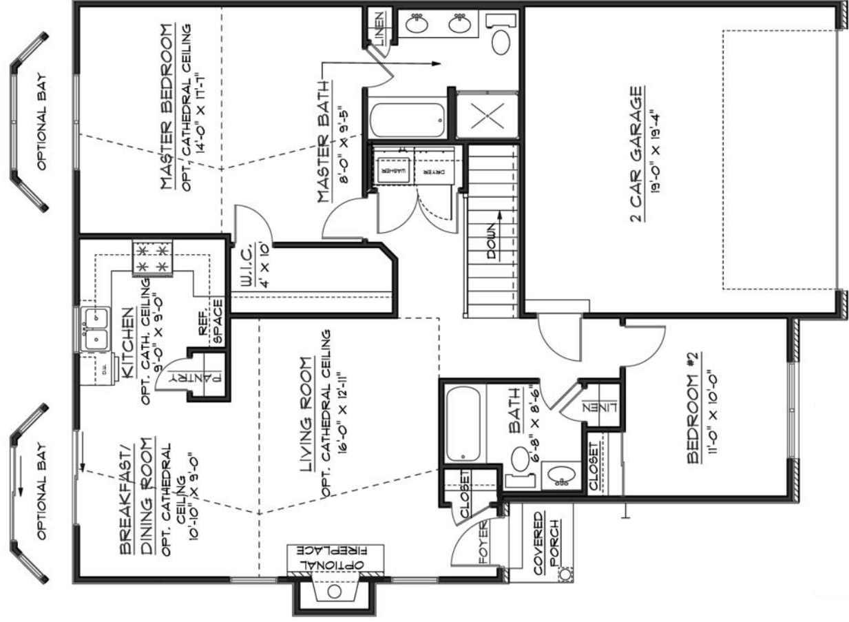
Optional with foundation floorplan
